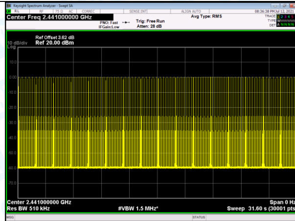
2441MHz DH3
