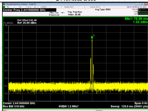
2441MHz DH3
