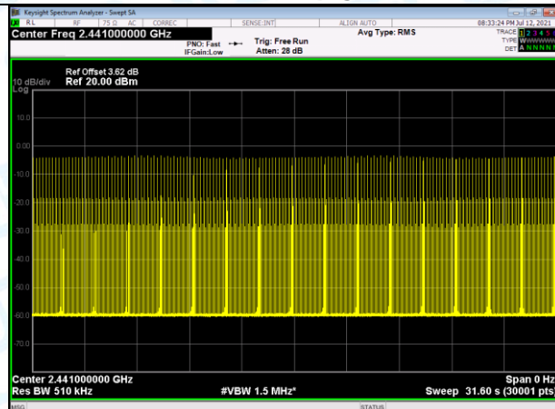
2441MHz 2DH5
