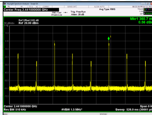
2441MHz 2DH5
