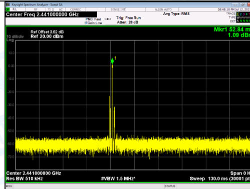
2441MHz 2DH3
