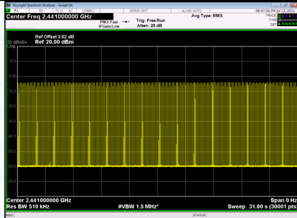
2441MHz 2DH3
