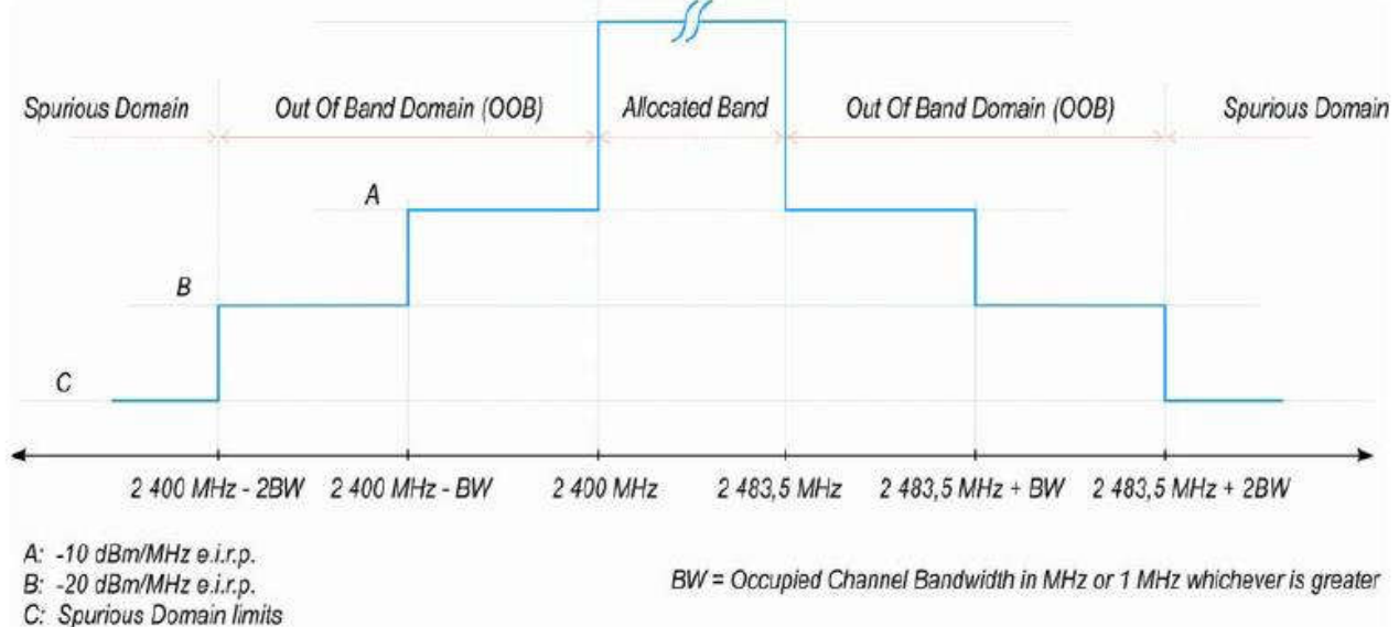
Figure 1: Transmit mask
